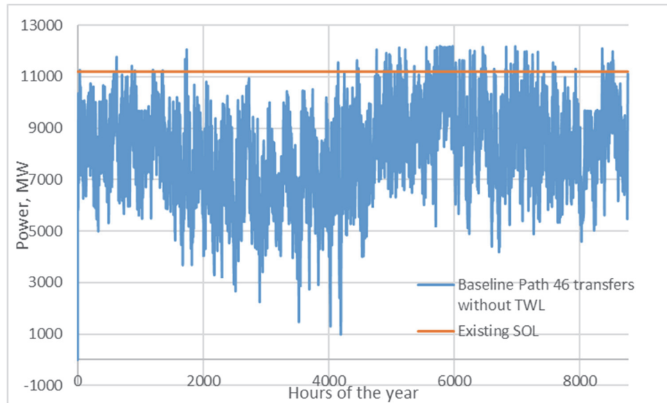
Figure 4: Projected Path 46 Transfers without Ten West Link in the Sensitivity Case
