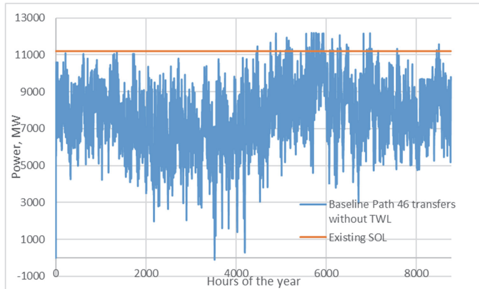
Figure 3: Projected Path 46 Transfers without Ten West Link in the Baseline Case
