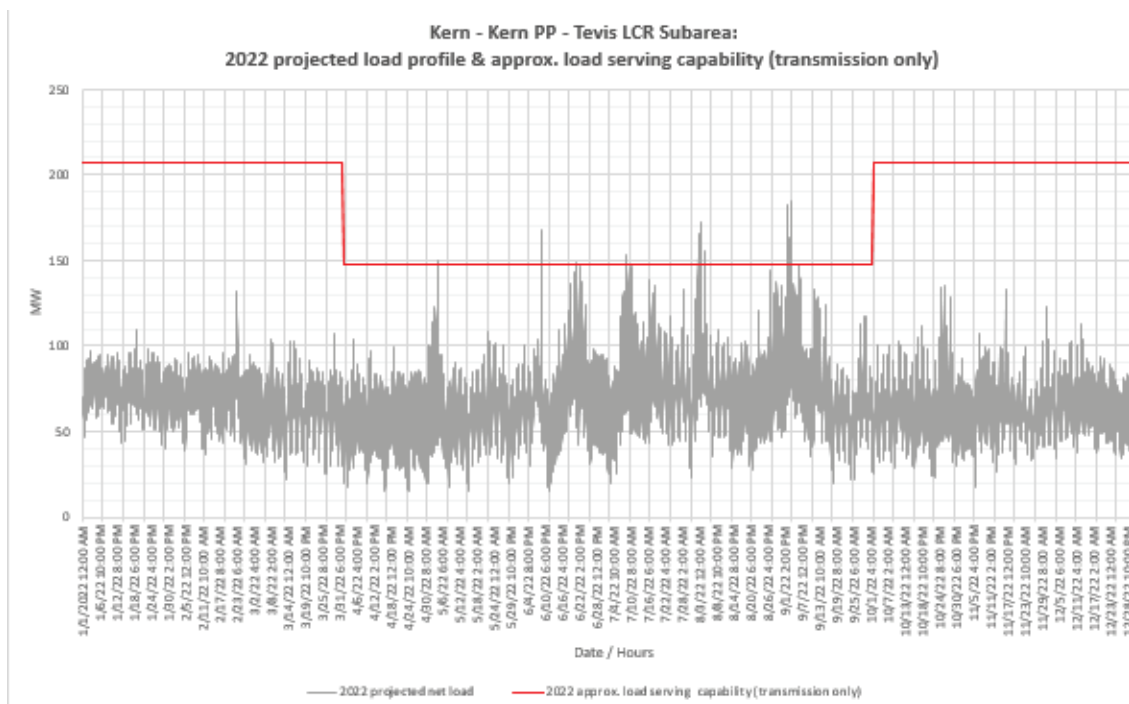
Figure 3.3-72 Kern Power- Tevis LCR Sub-area 2022 Forecast Hourly Profiles
