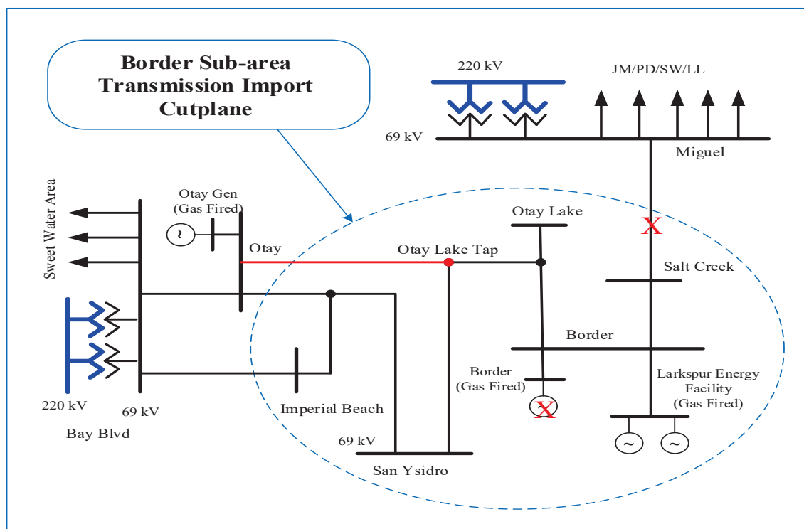
Figure 3.3-102 Border LCR Sub-area
