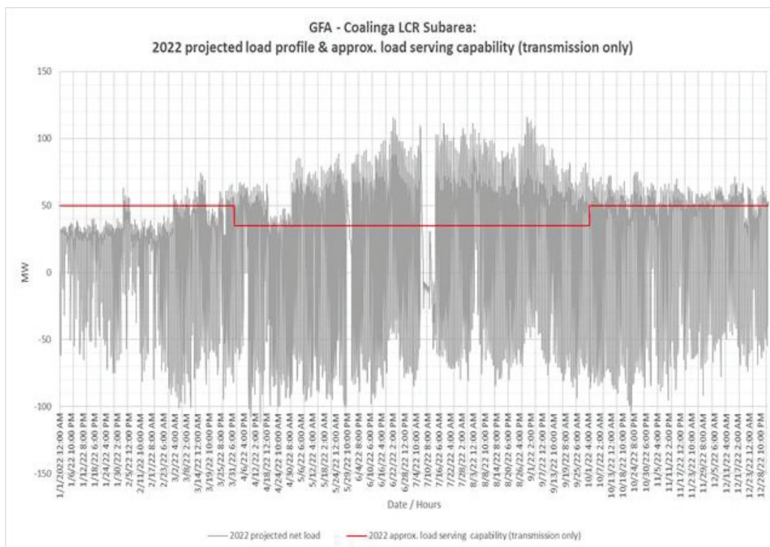
Figure 3.3-53 Coalinga LCR Sub-area 2022 Forecast Hourly Profiles
