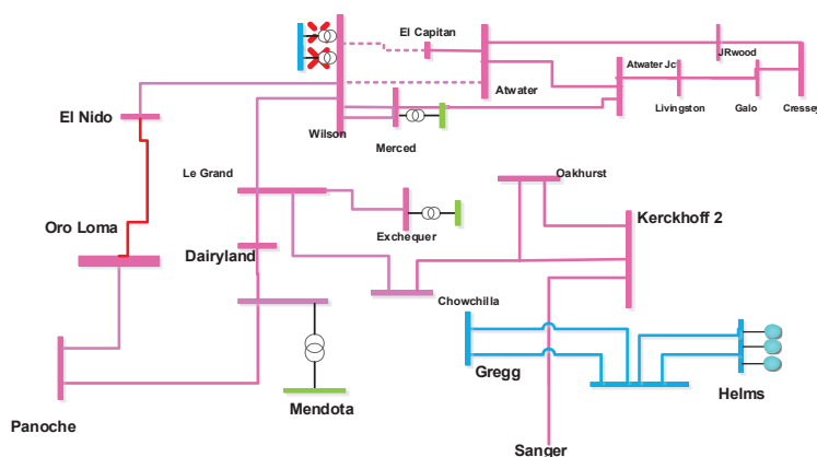
Figure 3.3-63 Wilson LCR Sub-area
