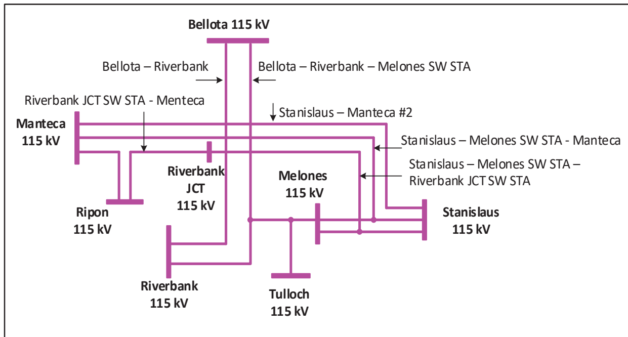
Figure 3.3-28 Stanislaus LCR Sub-area
