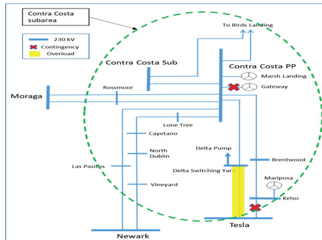
Figure 3.3-44 Contra Costa LCR Sub-area
