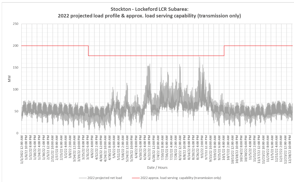
Figure 3.3-27 Lockeford LCR Sub-area 2022 Forecast Hourly Profiles
