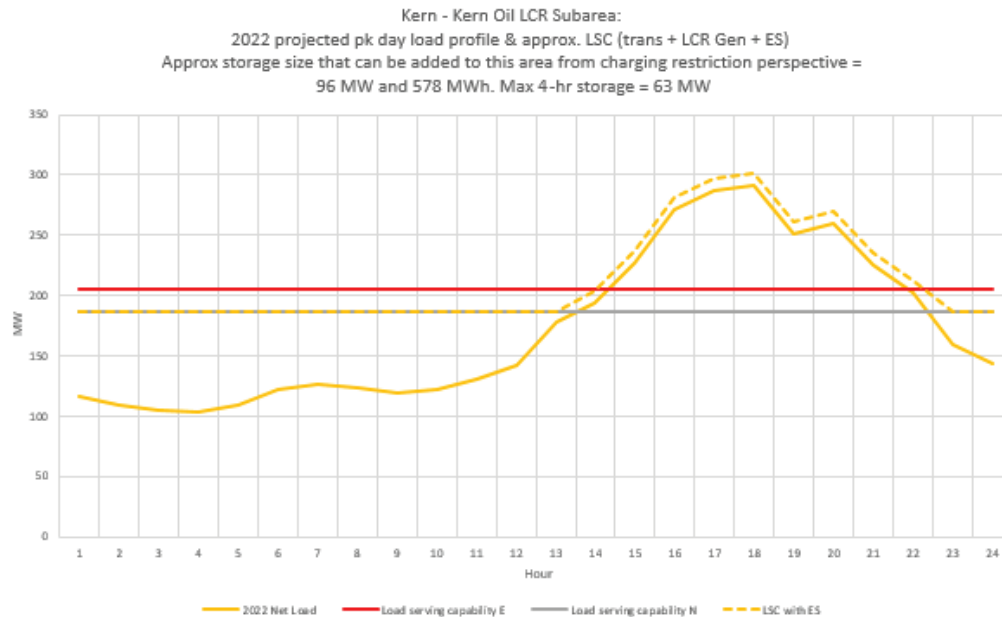
Figure 3.3-77 Kern Oil LCR Sub-area 2022 Forecast Hourly Profiles
