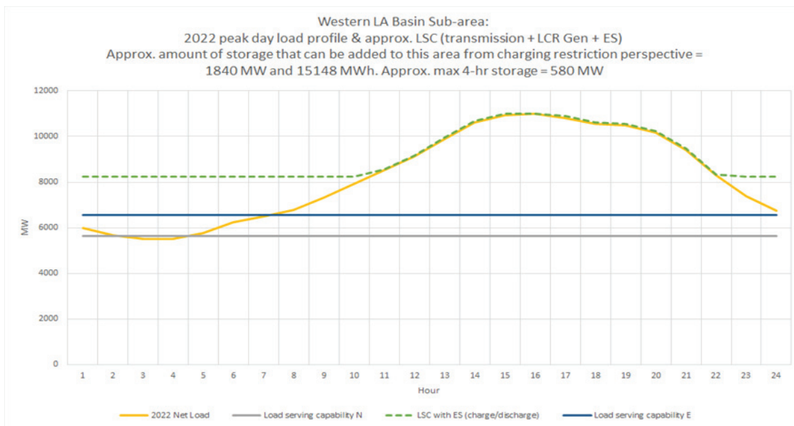
Figure 3.3-93 Western LA Basin LCR Sub-area 2022 Load Shape and Estimated Maximum Energy Storage Capacity and Energy Based on Charging Capability Under Critical Contingency
