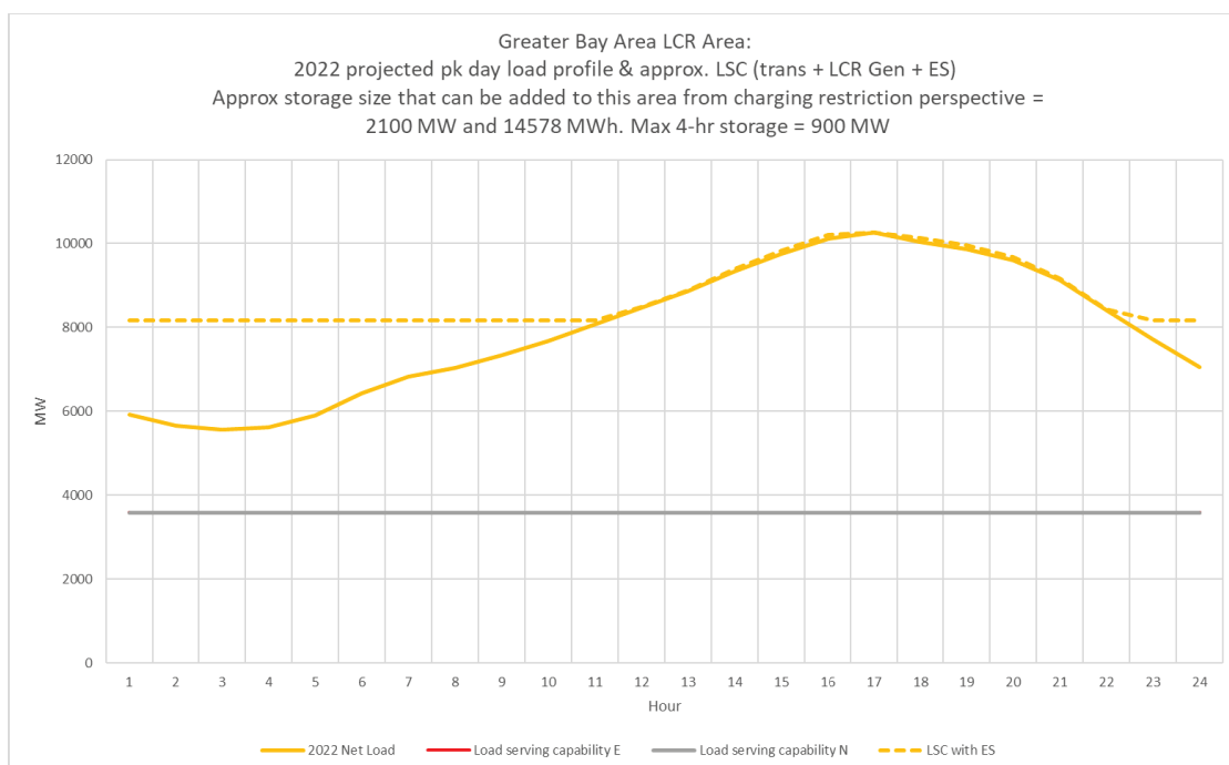
Figure 3.3-45 Bay Area LCR Area 2022 Peak Day Forecast Profiles
