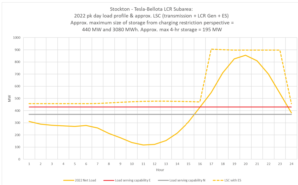
Figure 3.3-31 Tesla-Bellota LCR Sub-area 2022 Forecast Hourly Profiles
