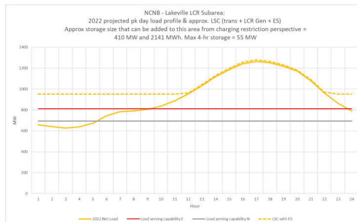
Figure 3.3-5 North Coast and North Bay 2022 Peak Day Forecast Profiles
