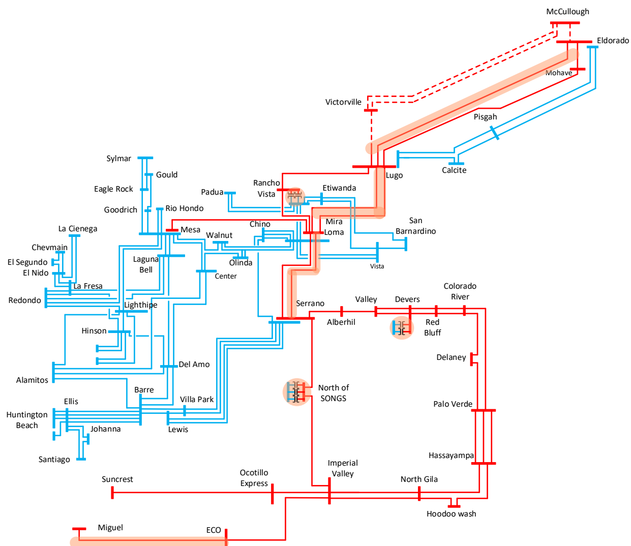
Figure 5-6: Overloads Identified in LA Basin 500 kV Study Area under N-1-1 Contingencies
