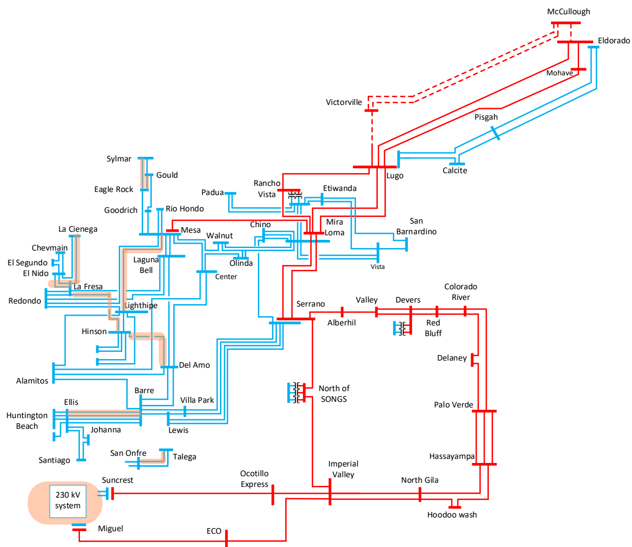
Figure 5-7: Overloads Identified in LA Basin 230 kV Study Area under N-1-1 Contingencies
