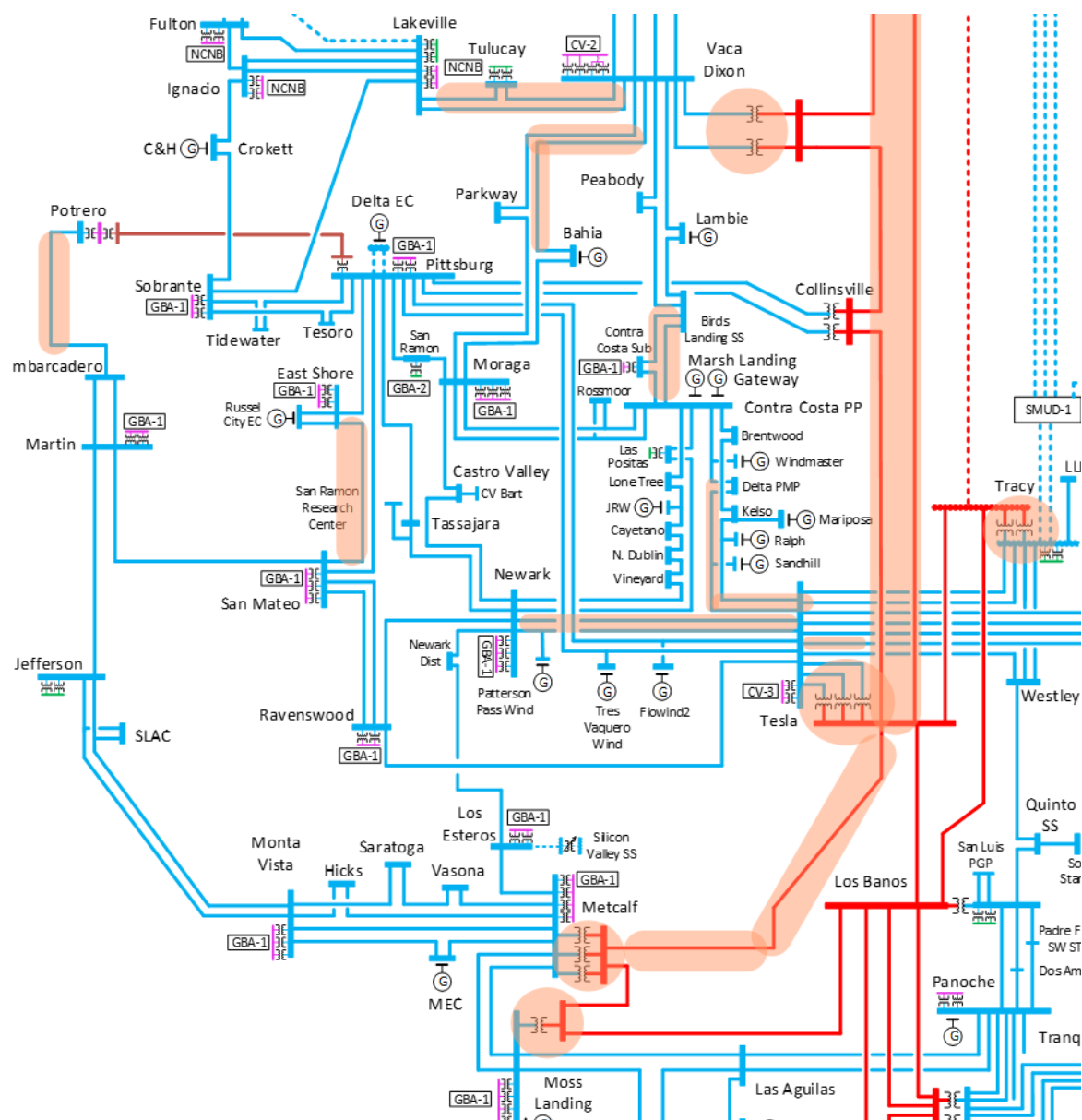
Figure 5-1: Transmission system in Bay Area and identified overloads under N-0 and N-1 Contingencies
