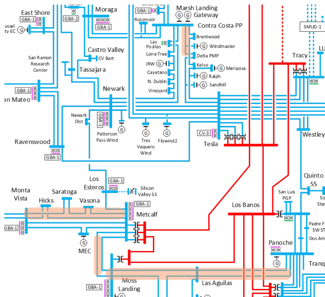
Figure 5-5: Overloads identified in Bay Area under N-1-1 Contingencies
