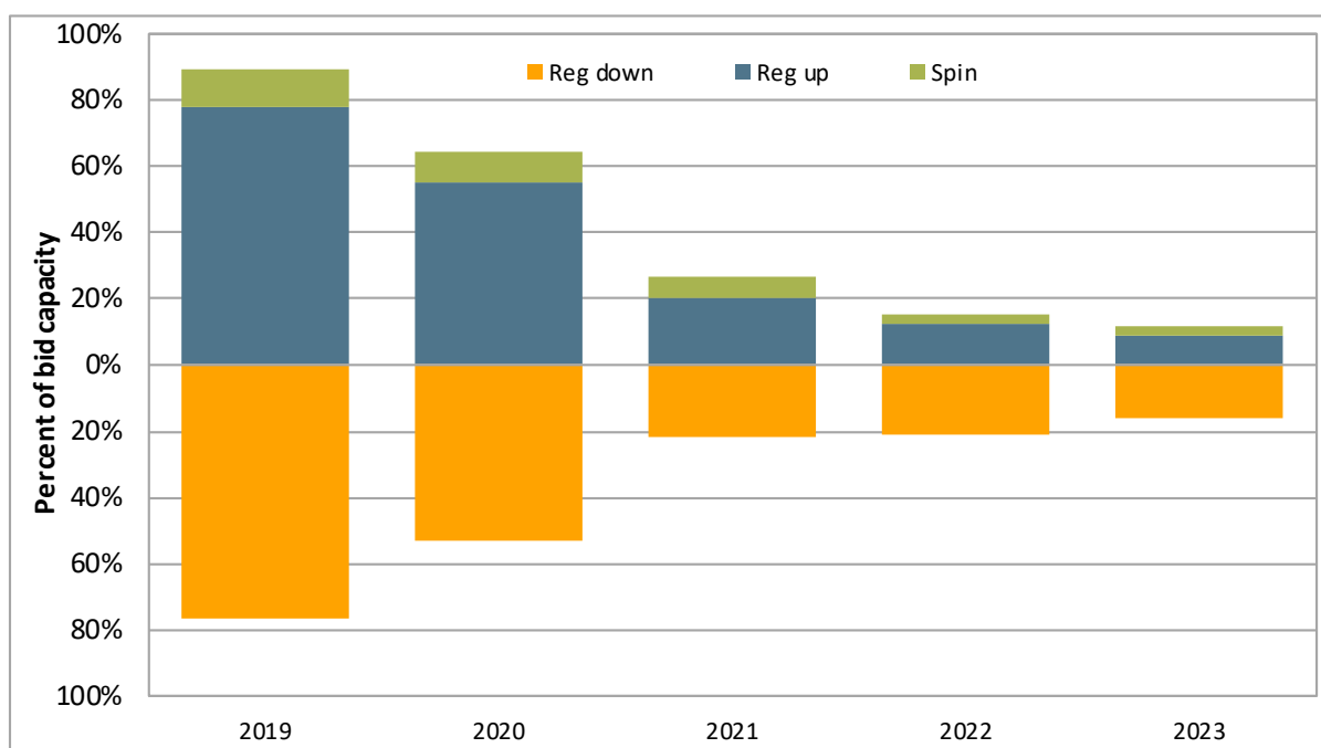
Figure 2.21 Percent of battery capacity scheduled for ancillary services
