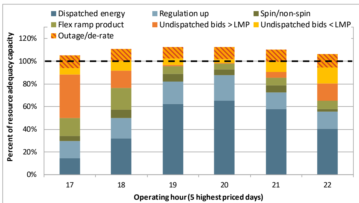
Figure 2.24 Average 15-minute resource adequacy battery capacity during 5 highest priced days
