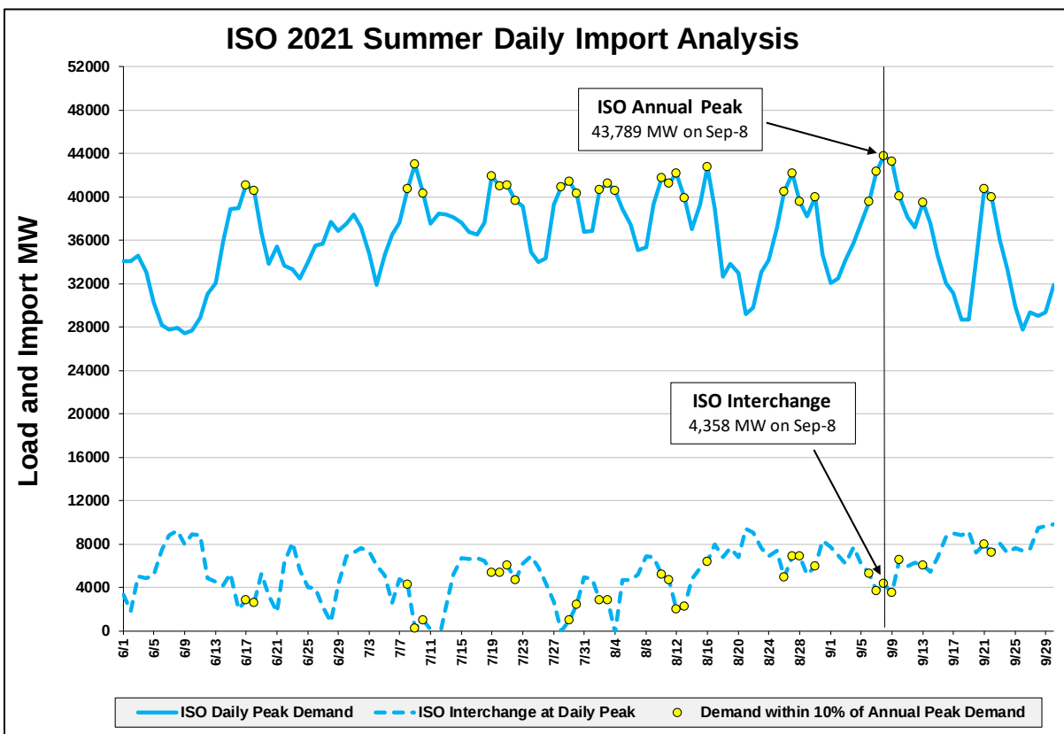
Figure 7 shows the amount of net imports at ISO 2021 daily system peaks.
