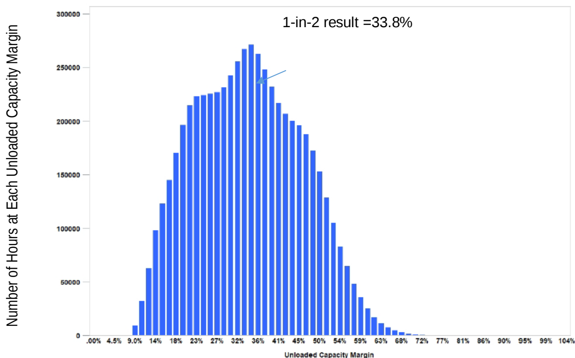
Figure 17 shows the distribution of the UCMs over all 2,928 summer operating hours from all 2,000 scenarios.
